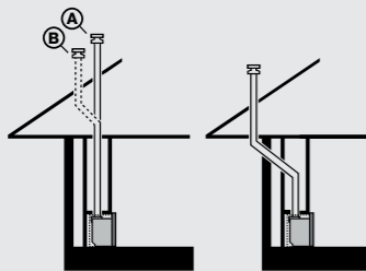
Inbuilt - Zero Clearance (Sapphire / Slimfire)
