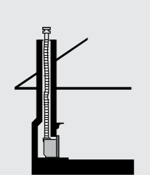
Inbuilt - Masonry (Sapphire / Slimfire)
