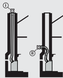
Masonry i. Vertical ii. Horizontal
