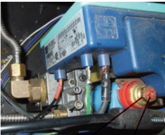
Max Pressure adjustment nut
